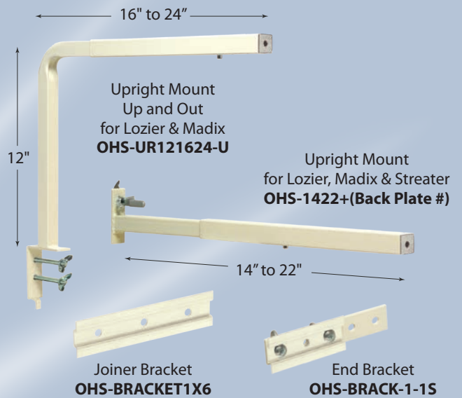
Adjustable Extension Arms
