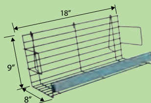
PGB-18x8x9-B 18" x 9" Angled Back Wire Shelf for Wine (Holds up to 12 Bottles)
