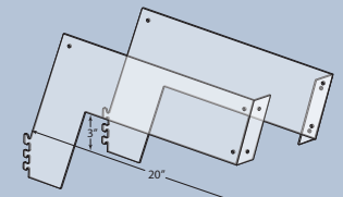
20" ANGLED Ghost Bracket
