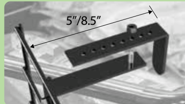
Adjustable Bracket to Fit Railings 5" to 8.5"
