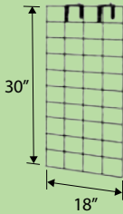
BG-A1830-B 18x30" Bunker Grid with 3" spacing, black, with adjustable 5-8.5" hanging brackets
