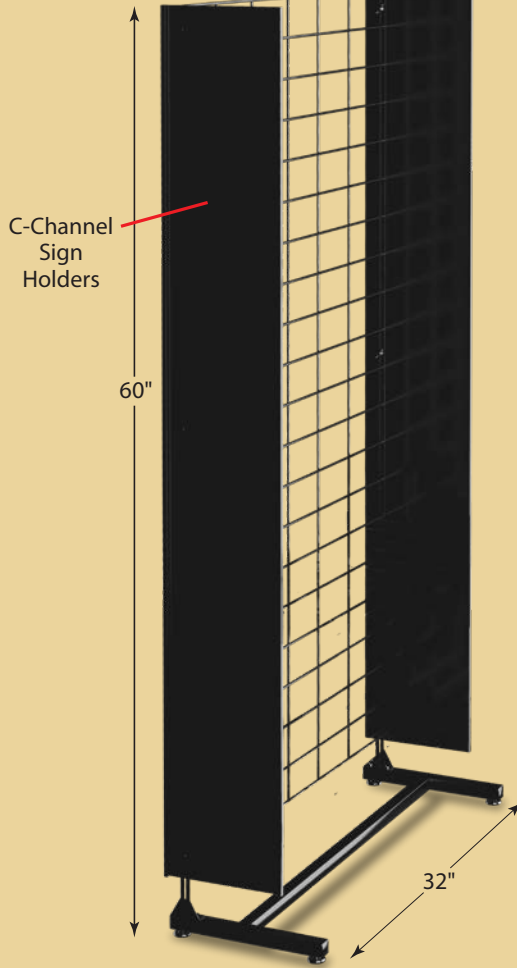
32" x 60" PowerGrid™ with 3" grid spacing With Casters PG-3260C-3-B With Levelers PG-3260L-3-B
