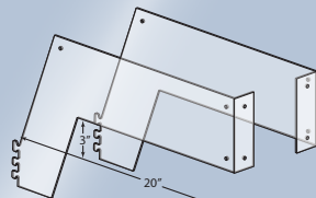
20" FLAT Ghost Bracket
