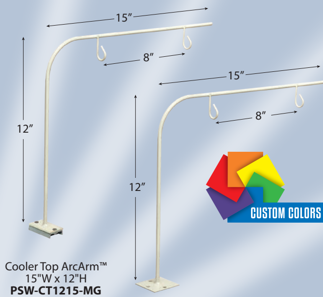
Cooler Top ArcArm™ Mount with 3 Screws 15"W x 12"H PSW-CT1215-CA
