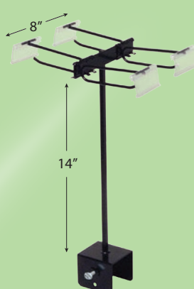
2.5" Clamp Mount 8" SpeedBar™ # PR-TC1408L-B
