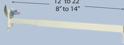
Adj. 3/4" PowerArm Single Slot w/DSU hwde. PP-1222DSU-34FFSL+(color) PP-814DSU-34FFSL+(color)
